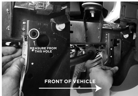
Fig. 2: NON-RUBICON(passenger side): Use the top 2 holes on the bracket to mount.
