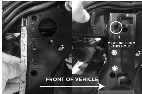
Fig. 1: RUBICON(passenger side): Use the bottom 2 holes on the bracket to mount.
