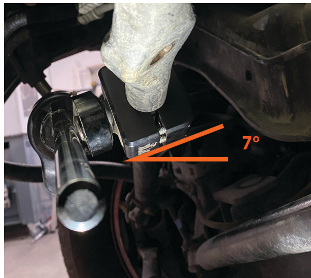
Fig. 5: Install the clamp at a 7 degree angle.
