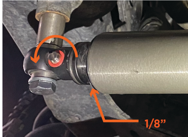
Fig. 2: Eyelet installed with 1/8" of shaft exposed.
