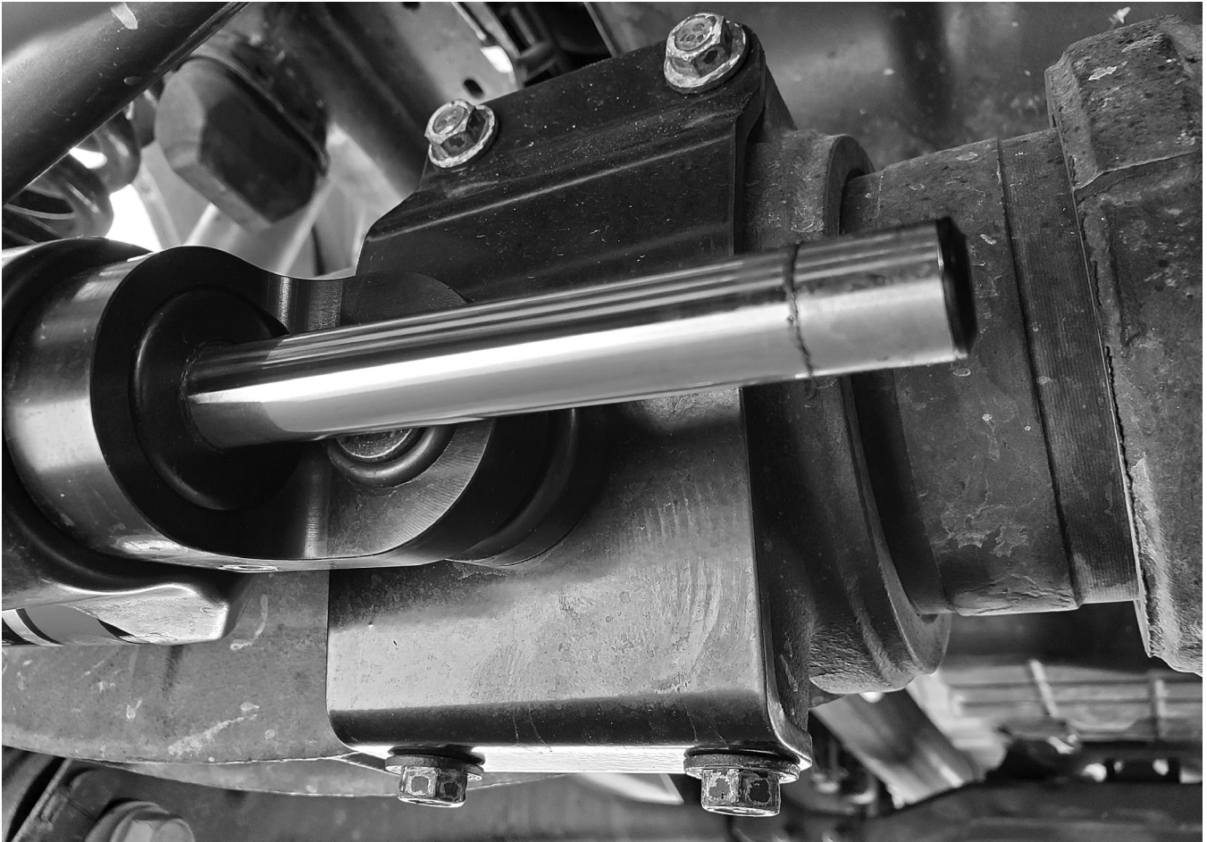
Figure 6: Axle bracket installed
