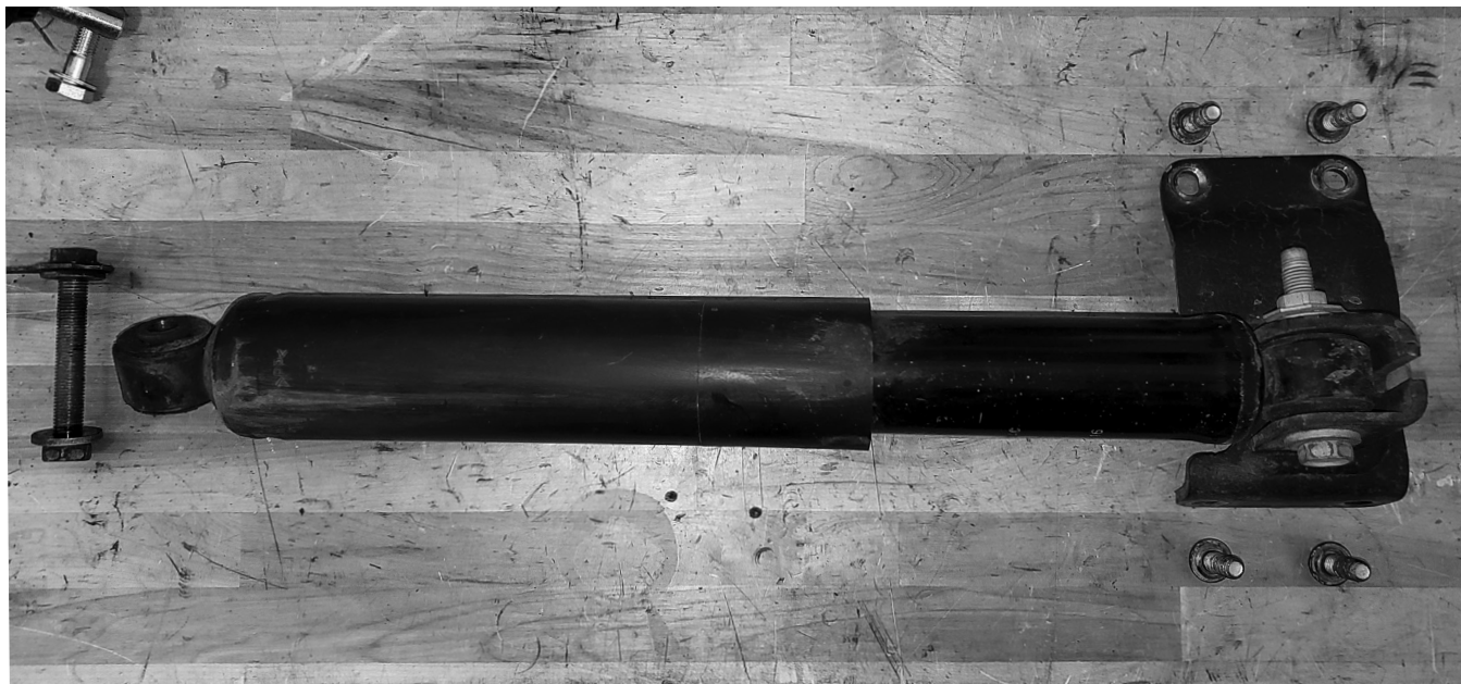
Figure 2: Stock hardware
