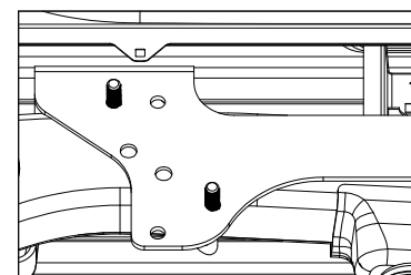
Figure D3: Short Bed U-bolt location.
